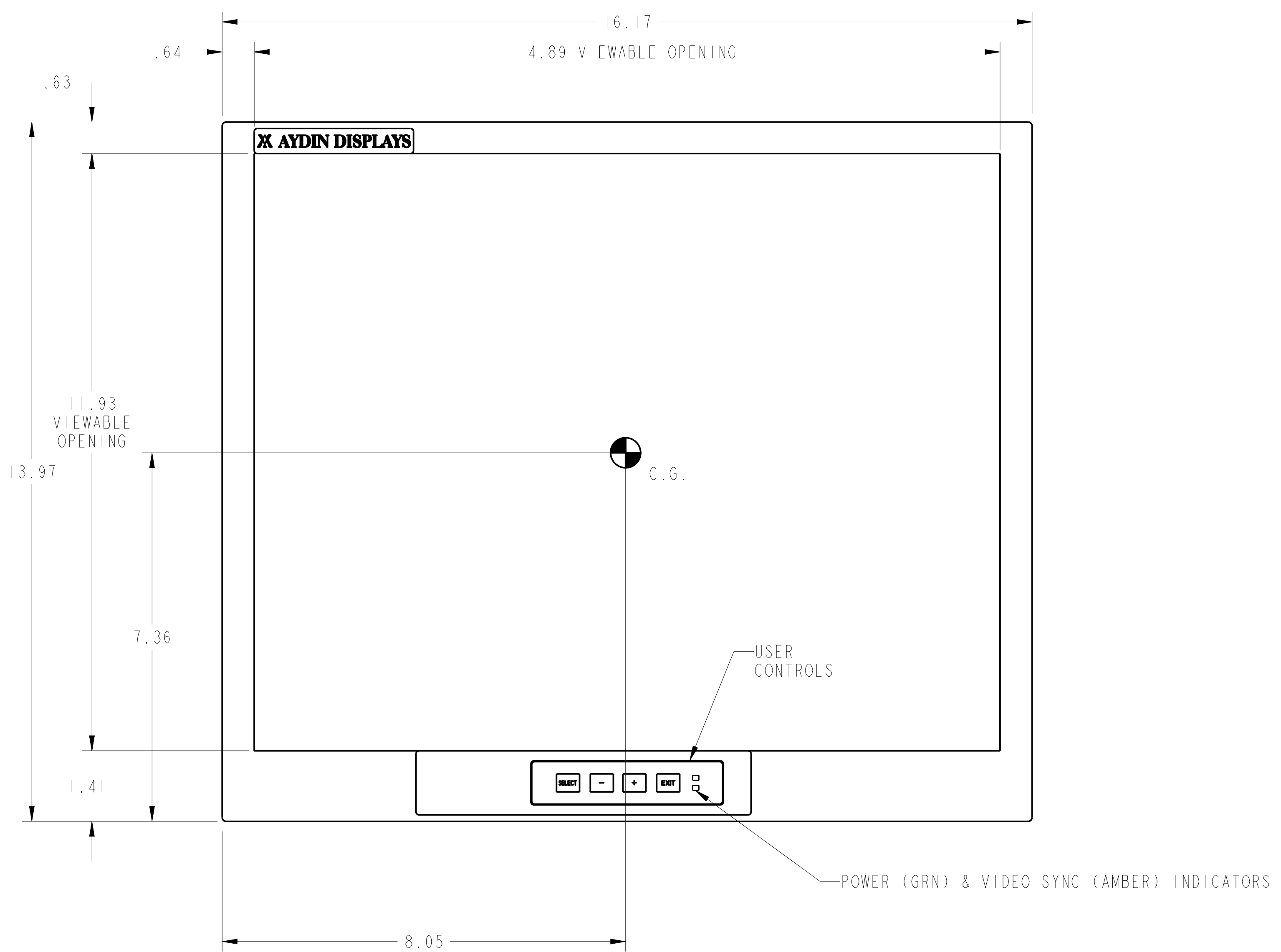
FRONT VIEW
