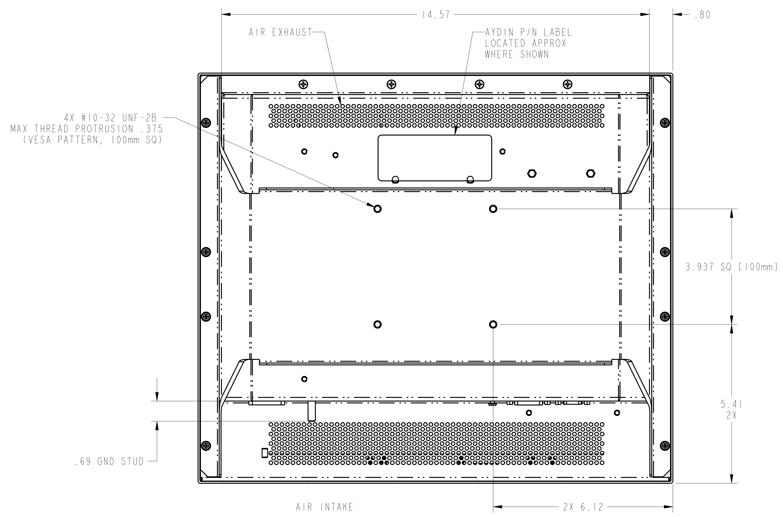
REAR VIEW
