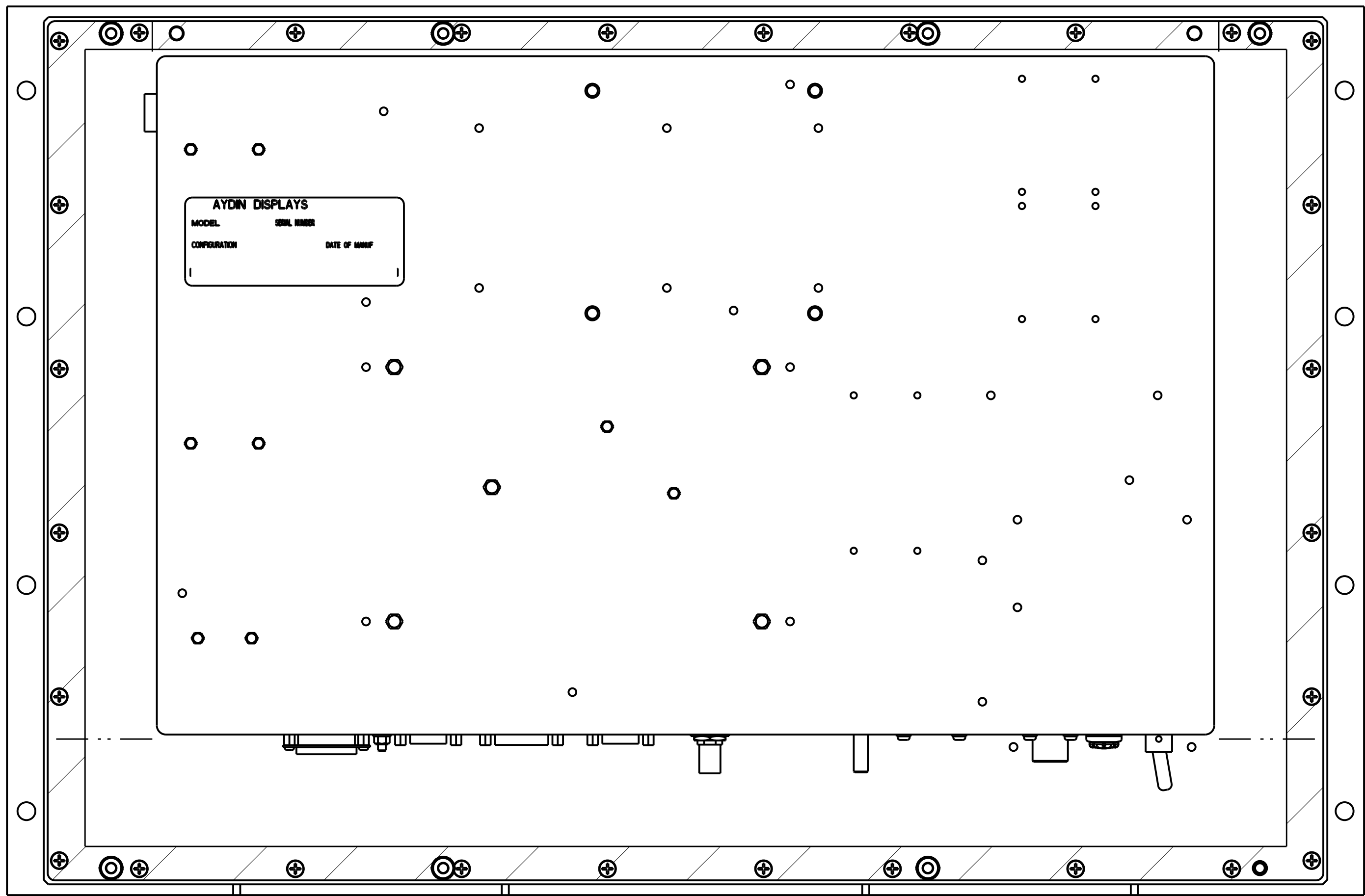
MODEL SHOWN WITH OPTIONAL FRONT RACK MOUNTING PLATE ASSY (351-00099) (P/N 356-7102-16XX)
